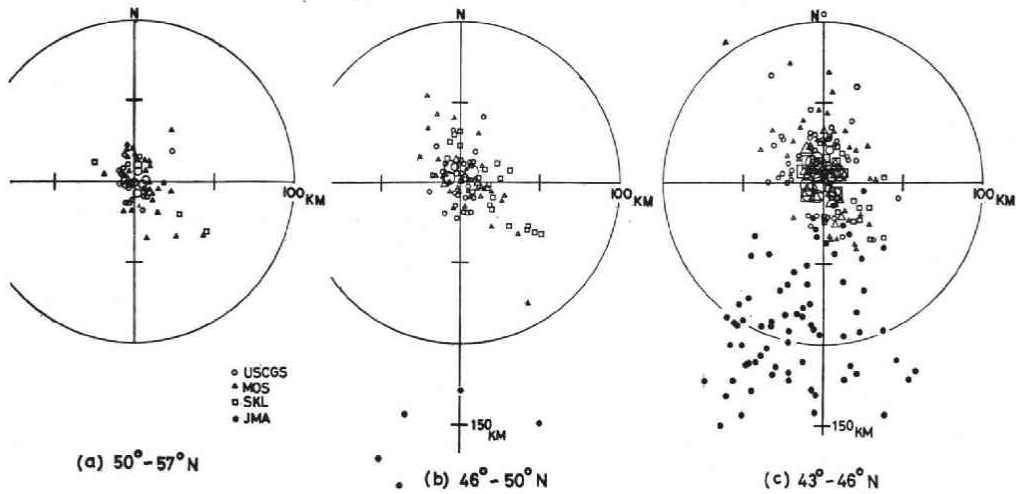
Fig. 1. Comparisons of the epicenter locations determined by I.S.C. with those by U.S.C.G.S., MOS, J.M.A., and S.K.L. The epicenters by I.S.C. are taken to be the origin of the coordinates for shallow earthquakes with magnitude greater than 5.0 in the period from 1964 to 1968. Symbol of small size; an epicenter for one shock. Symbol of medium size; epicenters for three shocks. Symbol of large size; epicenters for five shocks. Open circle; U.S.C.G.S. Solid circle; J.M.A. Triangle; MOS. Square; S.K.L.
