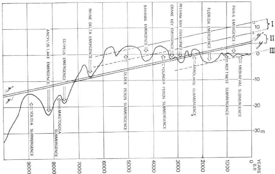
Fig. 6 Superposed uplift curve on Fairbridge's curve of sea level change
