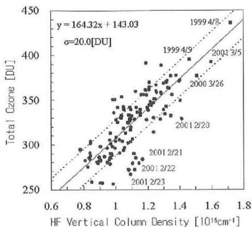
Fig. 1. Correlation of O_3 and HF.
