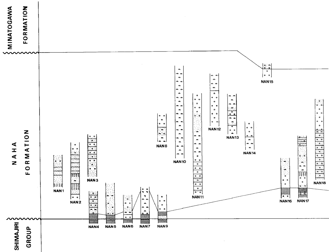
Fig. 30. Columnar sections of the Ryukyu
