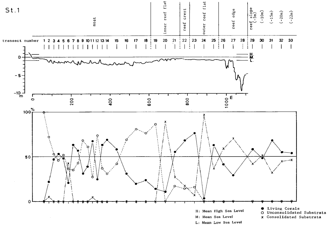
Fig. 9. Coverage rate of corals (●), unconsolidated substrata (○) and consolidated substrata (×) plotted against transect locations at St. 1.
