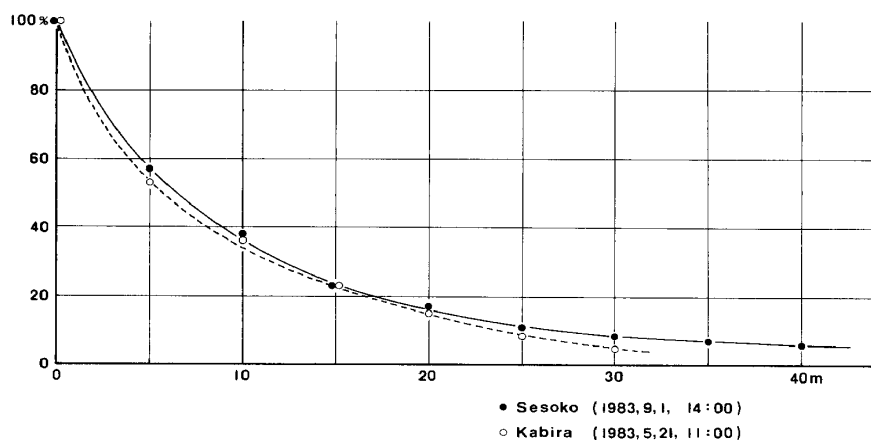
Fig. 5 Illumination intensity at St. 1 (○) and St. 4 (●). Horizontal axis indicates depth (m) and vertical axis relative illumination intensity to intensity in surface water (%).
