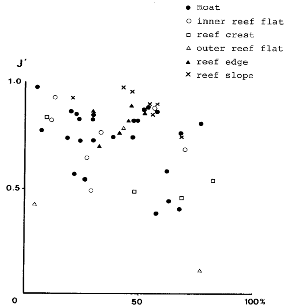
Fig. 24. Coral species equitability ( J' ) plotted against coral coverage in each topographic area.
