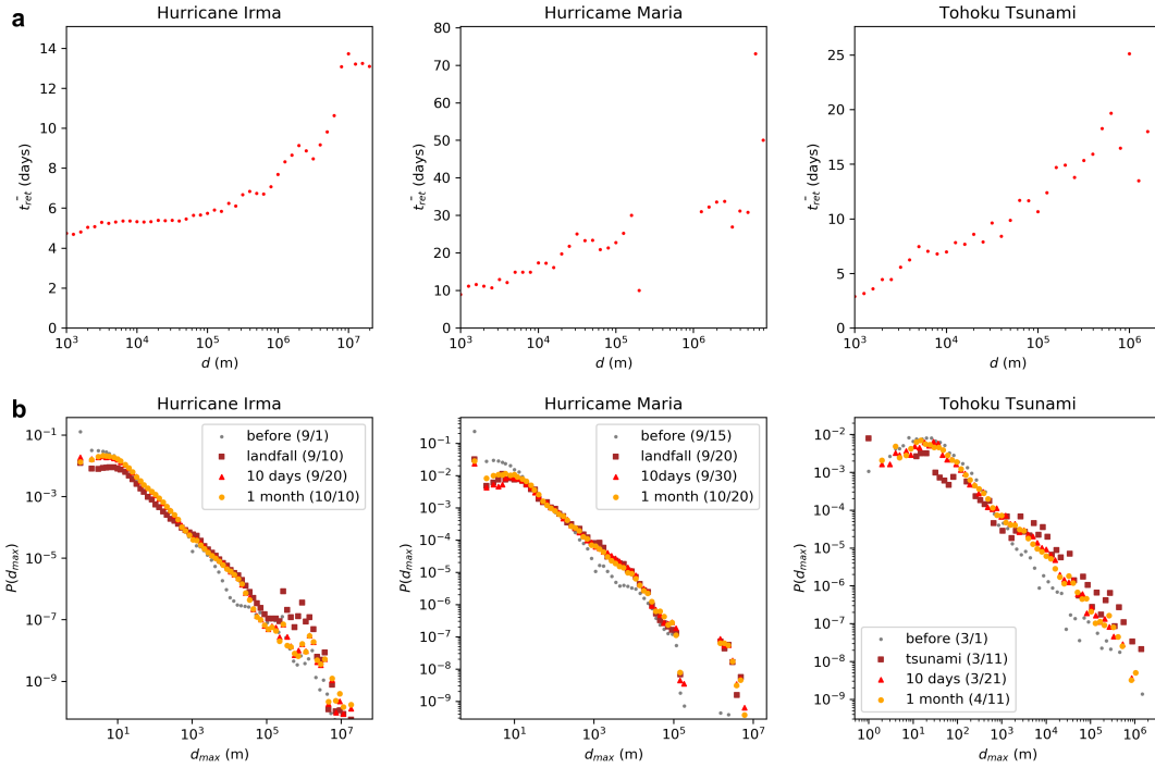
Figure 2: Relationship between displacement distance and duration after disasters. a. The longer the evacuation distance, the longer the average evacuation duration. b. Probability densities of maximum distance from home on a usual day (gray) and at various timings after the disaster day (brown: day of occurrence, red: 10 days after, orange: 1 month after) are all long-tailed. The long tailed distribution of evacuation distances and the relationship between displacement distance and duration were common across disasters. The majority of people evacuating short distances (thus short duration) and a small fraction of the people evacuating extremely long distances (thus long duration) explains why similar negative exponential functions were observed after the disasters.
