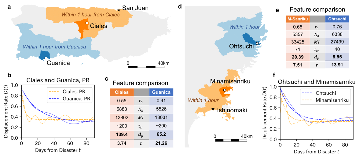
Figure 5: Connectedness to neighboring cities as a key factor to recovery. a. Map of Ciales and Guanica, Puerto Rico. Light colored areas show the area that can be reached from each city within one hour of driving time. b. Recovery patterns of both communities, showing the faster recovery of Ciales. c. Comparison of factors for both cities. Factors other than connectedness to other large cities (e.g. San Juan) were similar between the two communities. d-f. Similar phenomenon was seen after Tohoku Tsunami in Japan. Minamisanriku city and Ohtsuchi city shared similar characteristics except for the connectedness to large cities (e.g. Ishinomaki), resulting in differences in recovery patterns.
