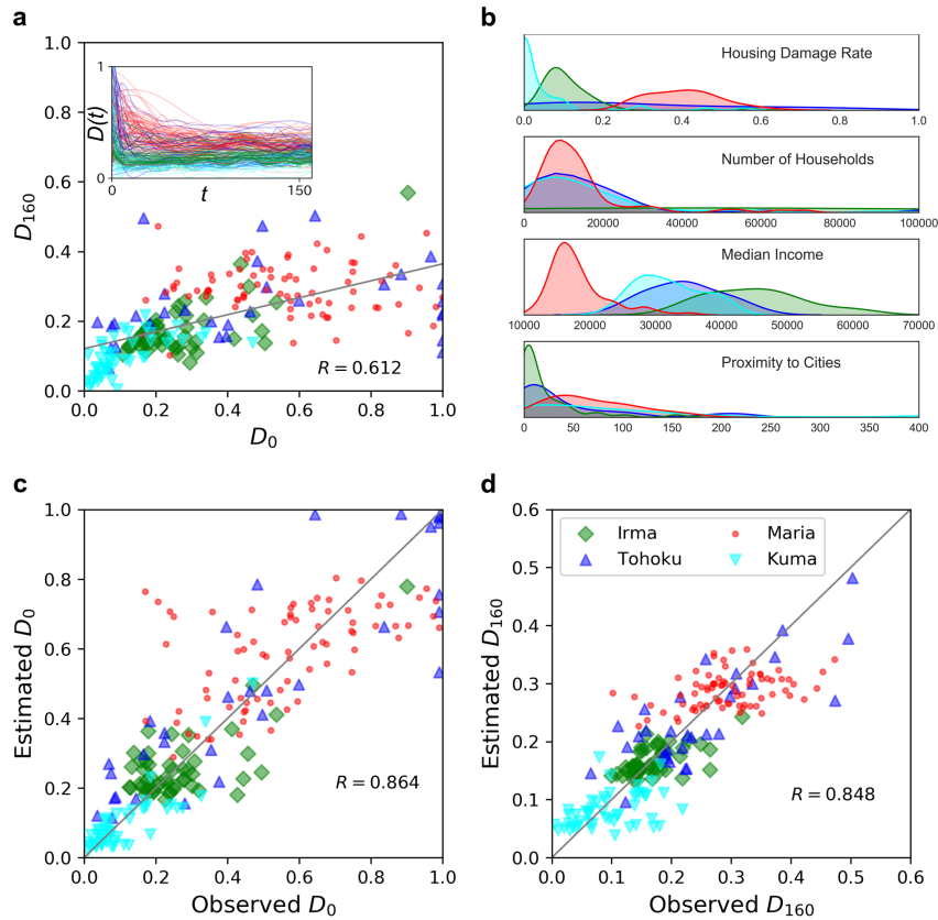
Figure 3: Explaining the spatial heterogeneity in population recovery using key common factors.
