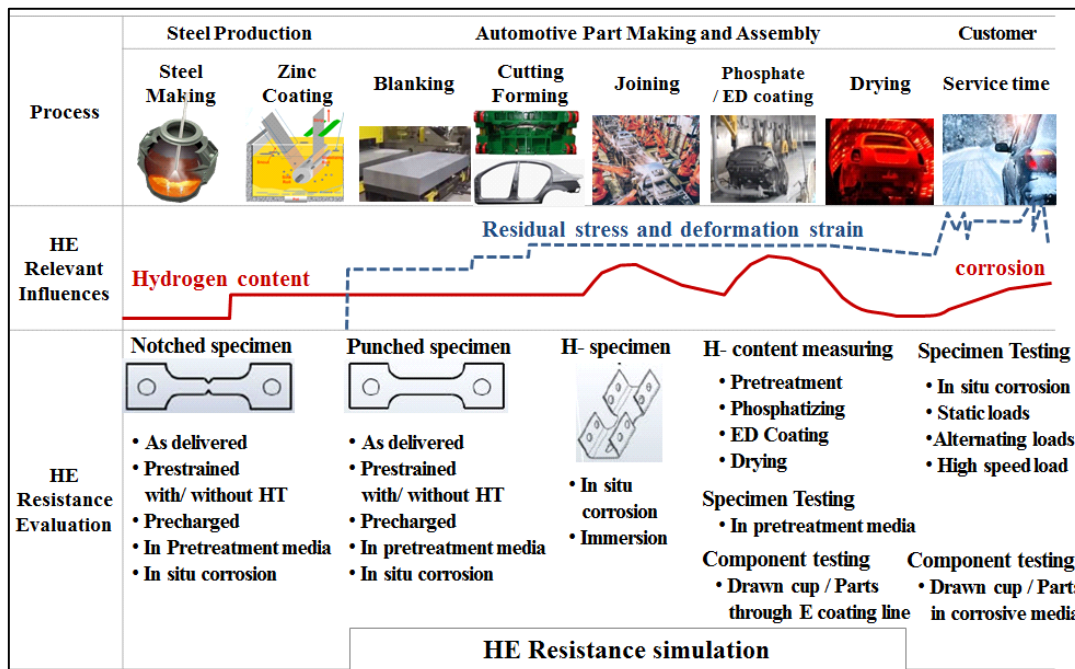
Figure. 1-17 Automotive part making process and simulation test method for HE [132].
