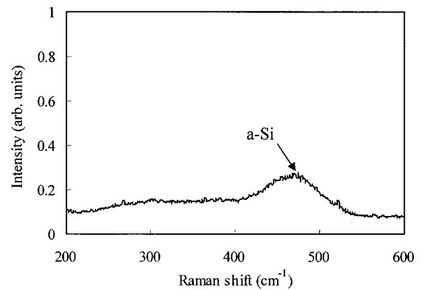
FIG. 8. Laser micro-Raman spectrum at an undeformed chip thickness of 200 nm. The broadband peak centered at 470\text{ cm}^{-1} is predominant, indicating that the subsurface layer within the measurement range has been almost completely transformed into the amorphous state.
