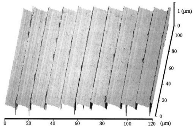
FIG. 4. Scanning laser microscopic topography of the machined silicon surface at an undeformed chip thickness of 200 nm, indicating a ductile–brittle transition machining regime.
