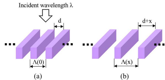
Fig. 1. Conceptual diagram of tunable wavelength-selective filters based on pitch-variable GR filters at (a) the initial state and (b) the expanding state. The d , \Lambda , and x show the initial groove width, the grating period, and the pitch variation, respectively.
