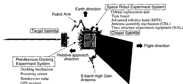
Figure 1: The Engineering Test Satellite VII
