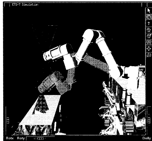
Figure 5: Example of the motion planning to a given goal with Zero Reaction Maneuver ( n = 7 )
