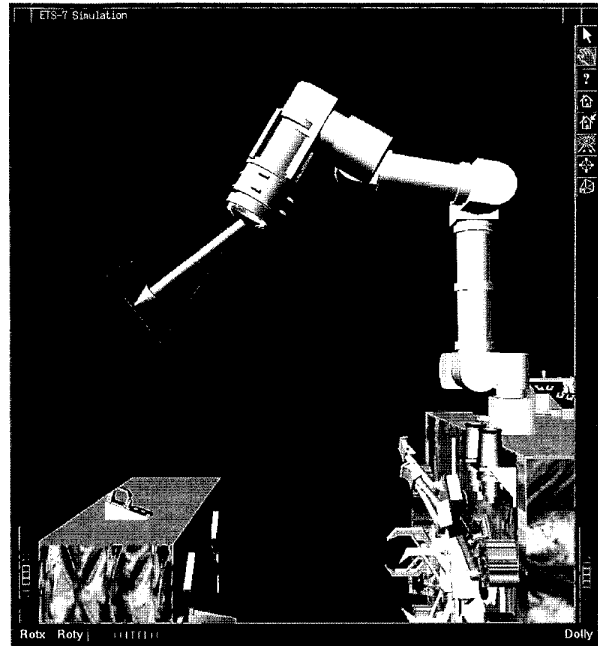
Figure 4: A plane for reactionless paths when n = 7
