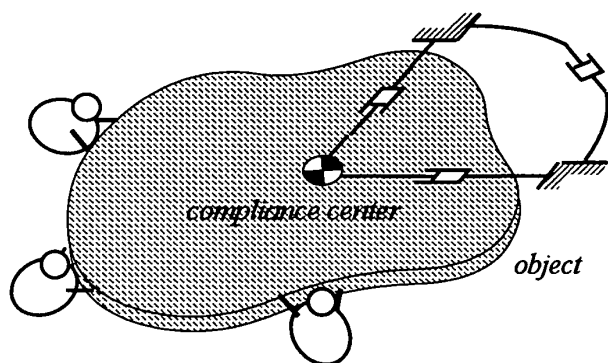
Fig. 6 3-DOF Damping Control
