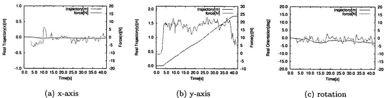
Fig. 11 Experimental Results (1-DOF Damping Control)
