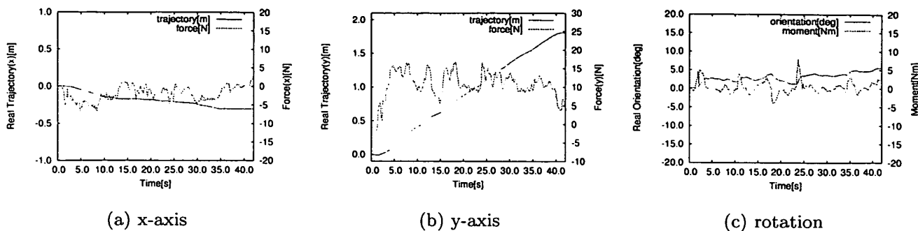
Fig. 10 Experimental Results (3-DOF Damping Control)
