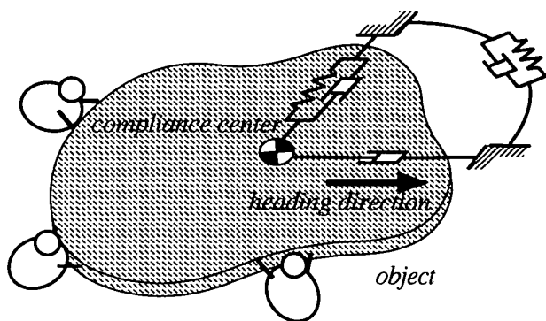
Fig. 7 1-DOF Damping Control
