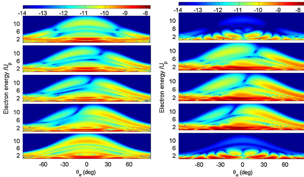
FIG. 3 (color online). Calculated angle-resolved ATI spectra for N_2 (left) and O_2 (right) for fixed orientation of the molecular axis for the intensities of Fig. 1. The orientation is at angles of \theta_L = 0^\circ, 30^\circ, 45^\circ, 60^\circ, and 90^\circ from top to bottom. For O_2 , we used \theta_L = 1^\circ and 89^\circ in place of 0^\circ and 90^\circ . For the latter angles, the rescattering plateau is entirely absent.
