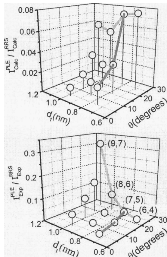
FIG. 1. Upper panel, calculated I_{\text{Calc}}^{\text{PLE}}/I_{\text{Calc}}^{\text{RRS}} intensity ratio; lower panel, experimental I_{\text{Exp}}^{\text{PLE}}/I_{\text{Exp}}^{\text{RRS}} intensity ratio, both for SWNTs with (2n+m)\bmod 3 equals 1 (type 1), as a function of diameter and chiral angle. The broad dark gray lines connect SWNTs with the same (2n+m) (similar d_i ) and the broad light gray lines connect SWNTs with the same (n-m) (similar \theta ). For each (2n+m)=\text{constant} family (similar d_i ), one (n,m) SWNT is assigned.
