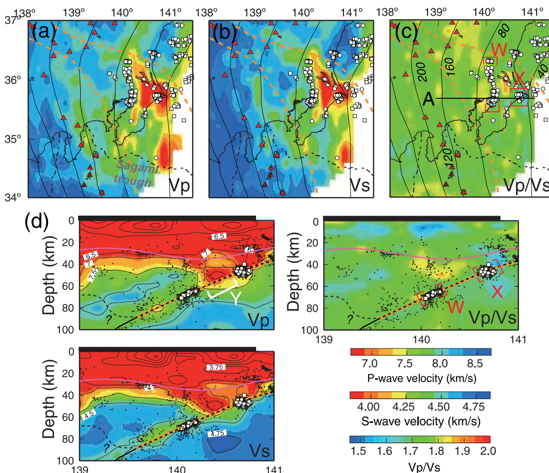
Figure 14. Seismicity along the upper surface of the PAC slab. Distributions of (a) P wave velocities, (b) S wave velocities, and (c) V_p/V_s ratios along the curved surface 5 km above the PAC slab. (d) East-west vertical cross sections of P and S wave velocities and V_p/V_s ratios along line A in Figure 14c. Isodepth contours of the PAC slab are shown by black lines with an interval of 40 km. White circles and squares denote interplate earthquakes and small repeating earthquakes, respectively, along the upper surface of the PAC slab. The seismicities labeled W and X in Figure 14c and the seismic gap of interplate earthquakes on the Pacific slab shown by Y in Figure 14d are discussed in the text. The other symbols are the same as in Figure 13.
