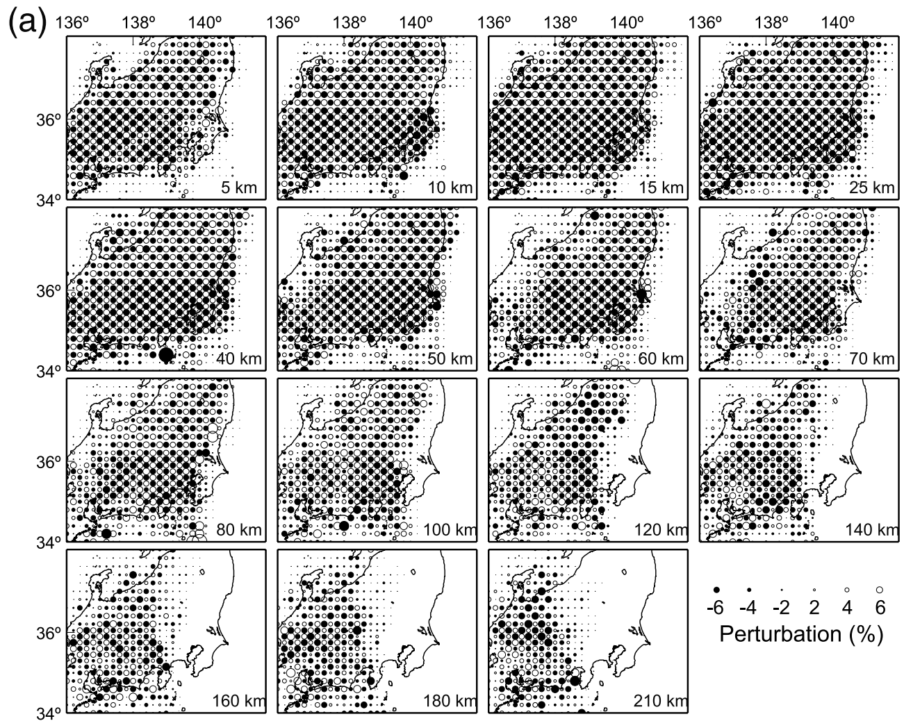
Figure B2. Results of the checkerboard resolution tests for (a) P and (b) S waves. Solid and open circles denote low and high velocities, respectively. The depth of the layer is shown at the bottom right corner of each panel.
