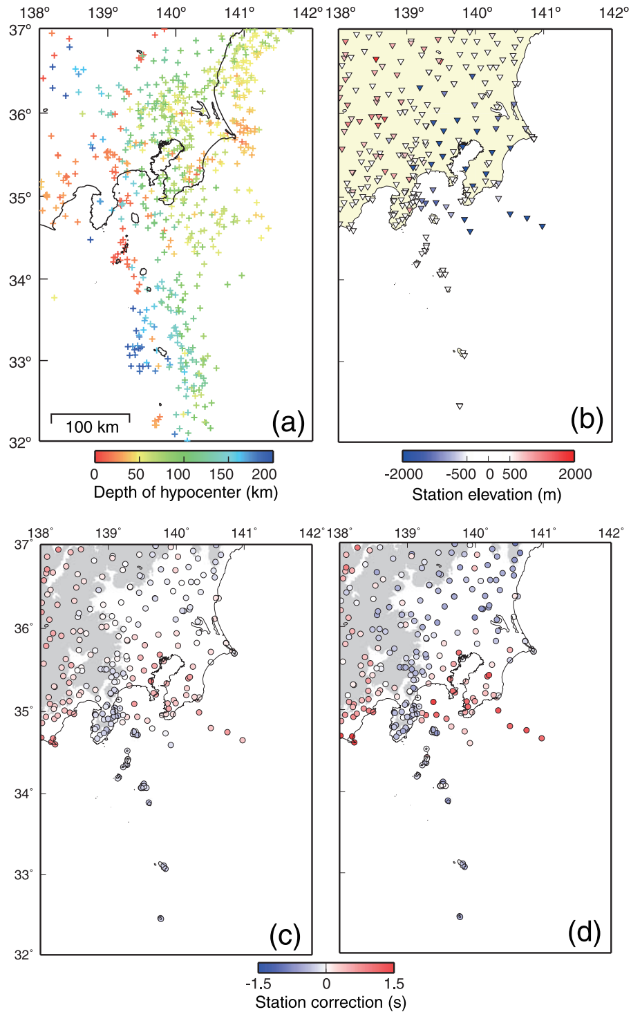
Figure A2. (a) Distribution of the 658 earthquakes used in the VELEST inversions. Colors represent the depths of hypocenters. (b) Distribution of seismic stations used in VELEST inversions. Colors represent the station elevations relative to the sea level. (c) Station corrections for P waves. (d) Station corrections for S waves. Gray areas in Figures A2c and A2d denote the areas with elevations of >500 m.
