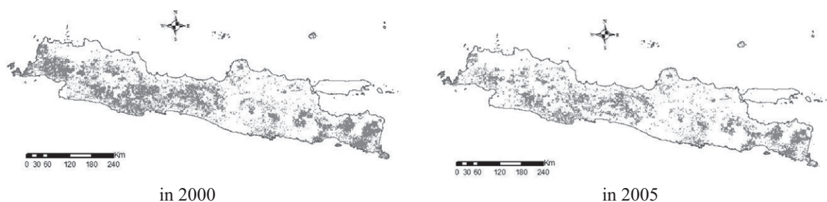
Fig. 1. Forest condition of Java Island in 2000 and 2005
