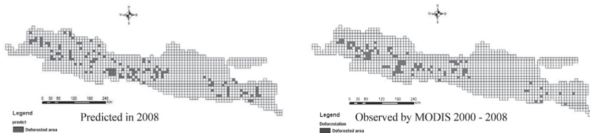
Fig. 6. Comparison of deforested and un-deforested areas predicted in 2008 and observed deforestation by MODIS 2000-2008
