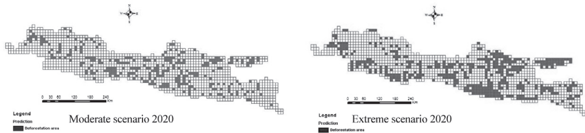
Fig. 4. Deforestation prediction in moderate and extreme scenarios in 2020
