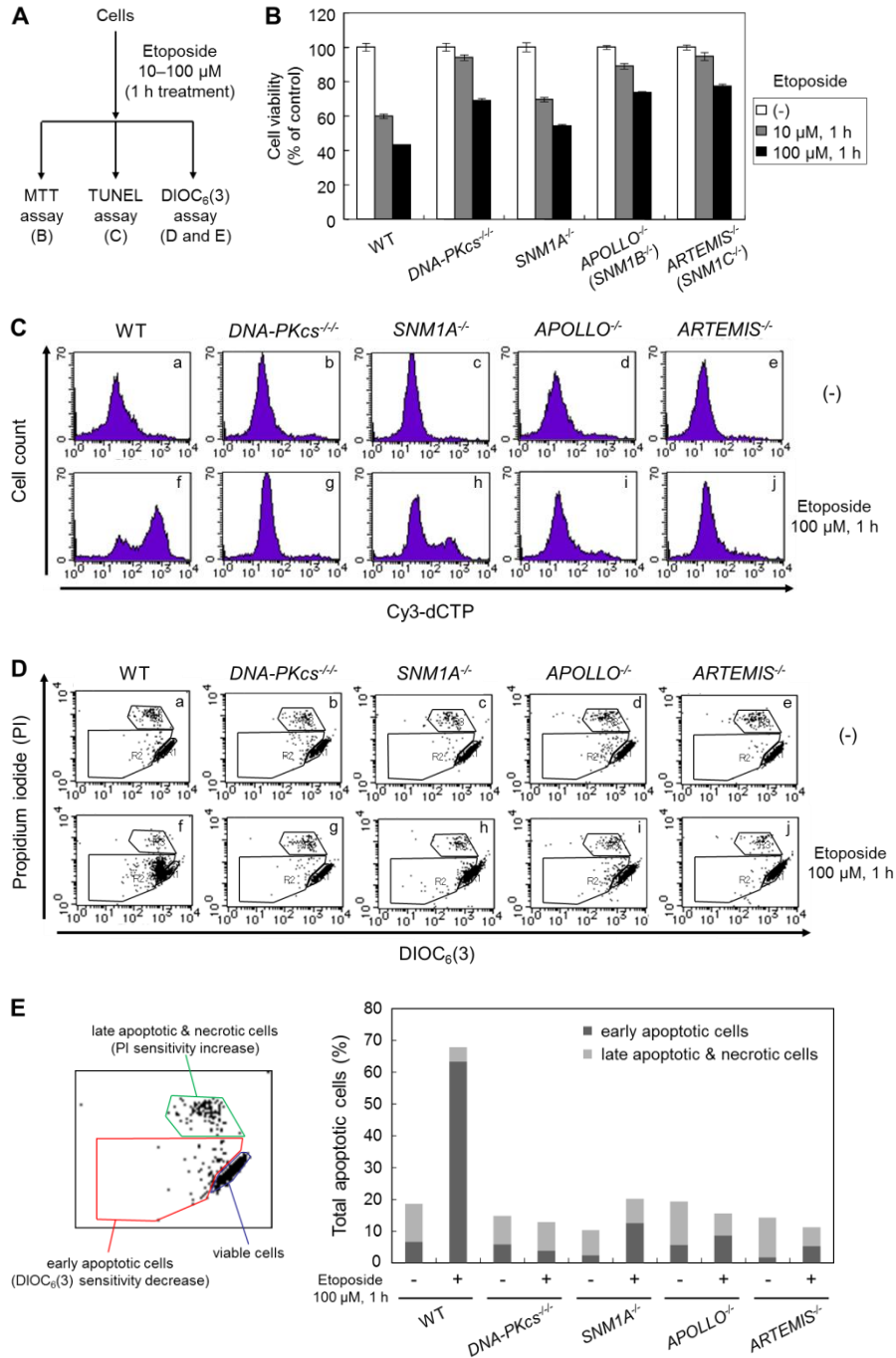
Fig. 4-1 Involvement of SNM1 family nucleases in the rapid induction of apoptosis by high doses of etoposide. (A) Scheme for experiments shown in Figure 1 B-E. (B) Cell viability measured by MTT assay. Cells were incubated for 1 h in the presence or absence of 10 or 100 μM etoposide, and their viability was measured by MTT assay. (C) Detection of DNA fragmentation by TUNEL. Etoposide-treated cells were fixed, and the termini of fragmented DNA were labeled with Cy3-dCTP. The TUNEL signal was measured by flow cytometry. (D and E) Detection of changes in mitochondrial membrane potential with DIOC6(3). Etoposide-treated cells were mixed with 3,3'-dihexyloxycarbocyanine iodide (DIOC6(3)) and propidium iodide (PI) to detect changes in the mitochondrial membrane potential and to distinguish early apoptotic cells from late apoptotic and necrotic cells. Cells were analyzed by flow cytometry (D). Quantification of the data shown in Figure 1D (E).
