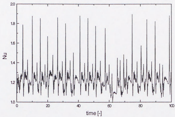
Fig. 4-7 Oscillation of Nu when R_c=100 , Le=10 and N=0.59
