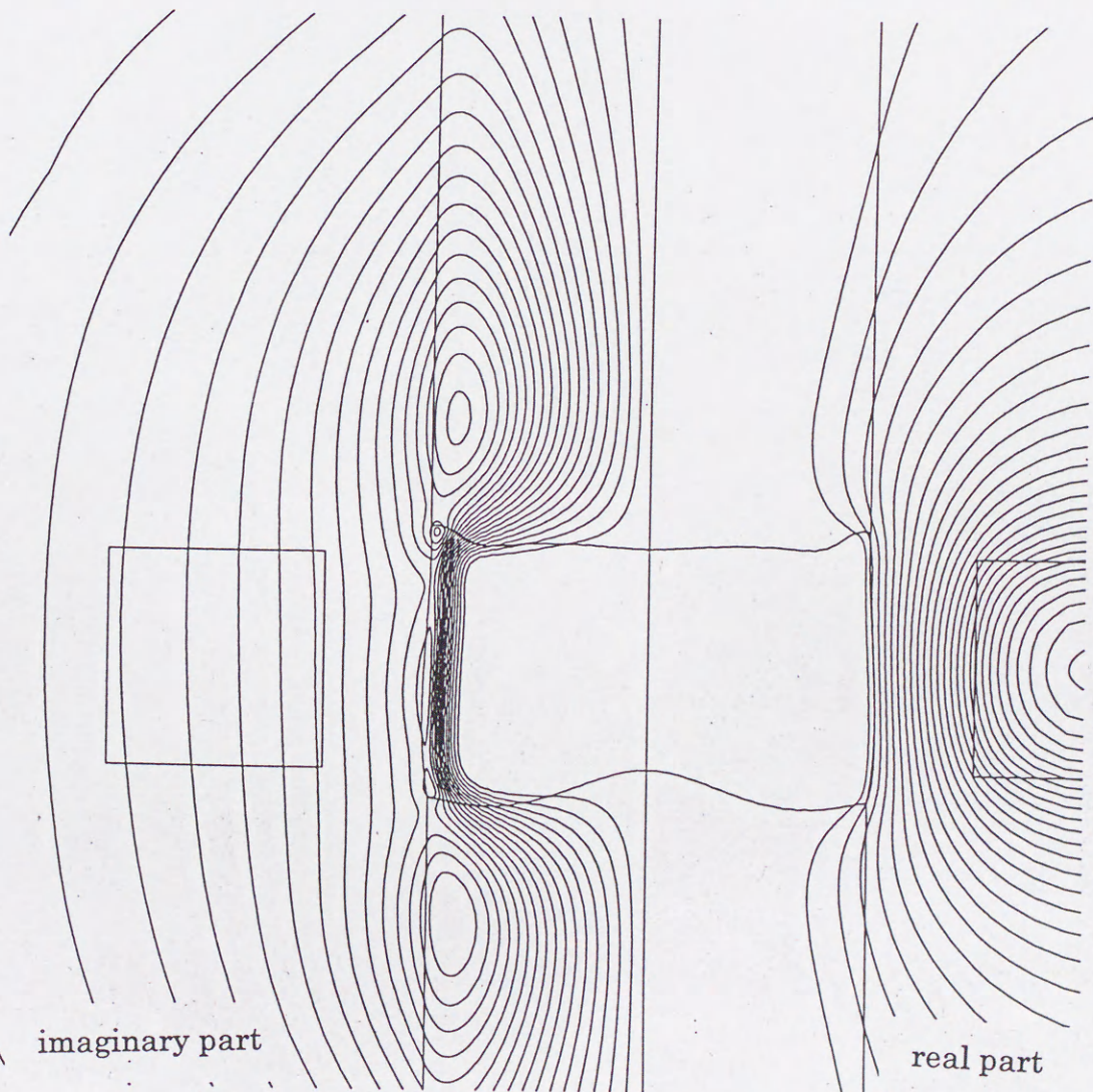
Fig.3-10 Electromagnetic fields in the FZ system when J_c'=1.4 \times 10^7 \text{ A/m}^2 and \omega=1.4 \text{ MHz}
