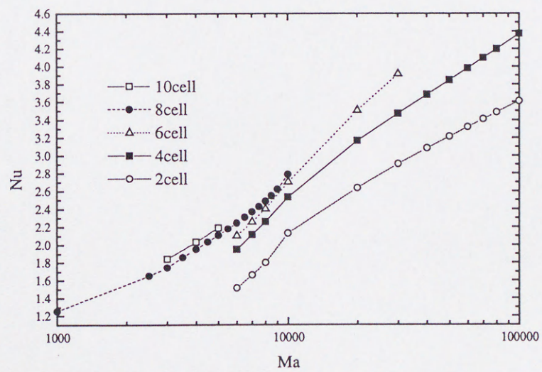
Fig.2-5 Ma vs Nu without inner heating for each convection pattern
