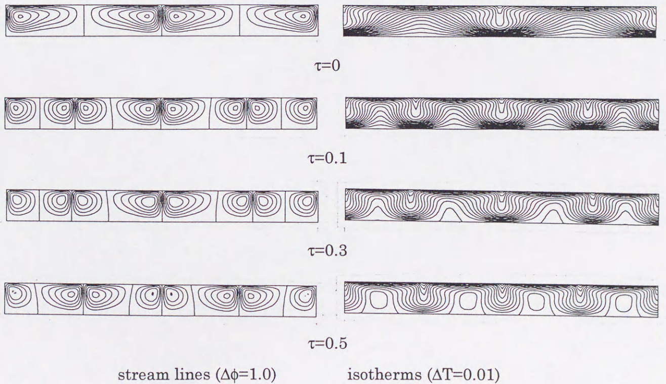
Fig.2-10 Stream lines and isotherms when Ma=6.0 \times 10^3 .
