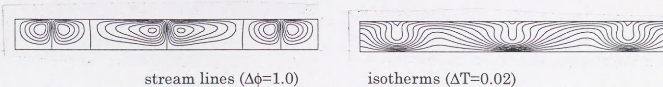
Fig.2-7 Stream lines and isotherms for Q=0 for Ma=5.0 \times 10^3 and Q=0 .
