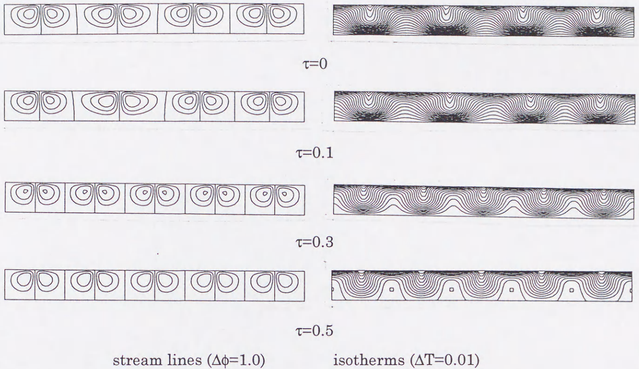
Fig.2-9 Stream lines and isotherms field when Ma=3.0 \times 10^3 .
