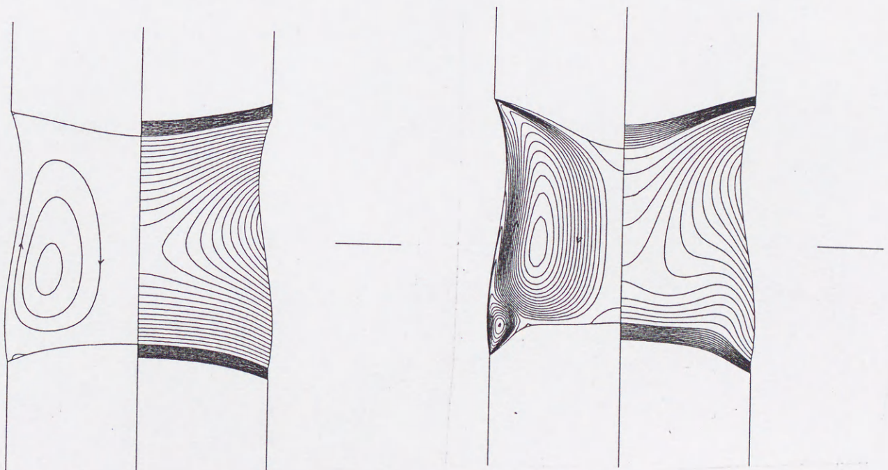
Fig. 3-3 Stream lines and isotherms in the melt zone when T_p=1.5 and \text{Pe}=0 .
