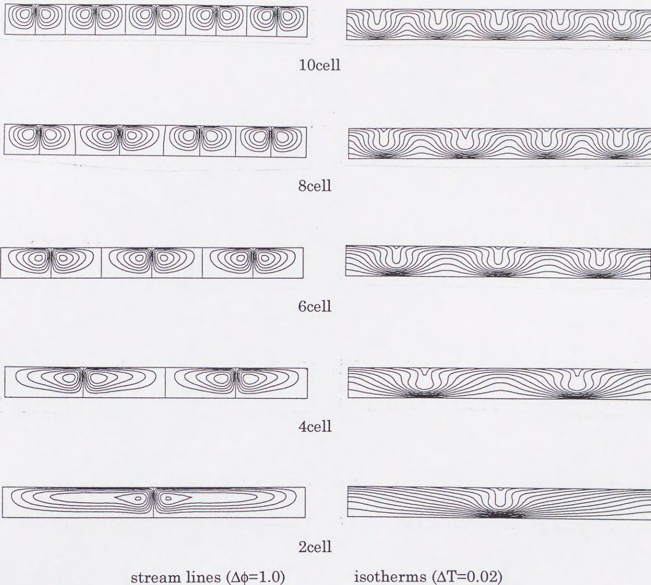
Fig.2-6 Stream lines and isotherms for Q=0 (10cell,8cell and 6cell when Ma=5.0 \times 10^3 , 4cell and 2cell when Ma=6.0 \times 10^3 )
