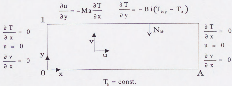
Fig.2-2 Physical model of the calculation
