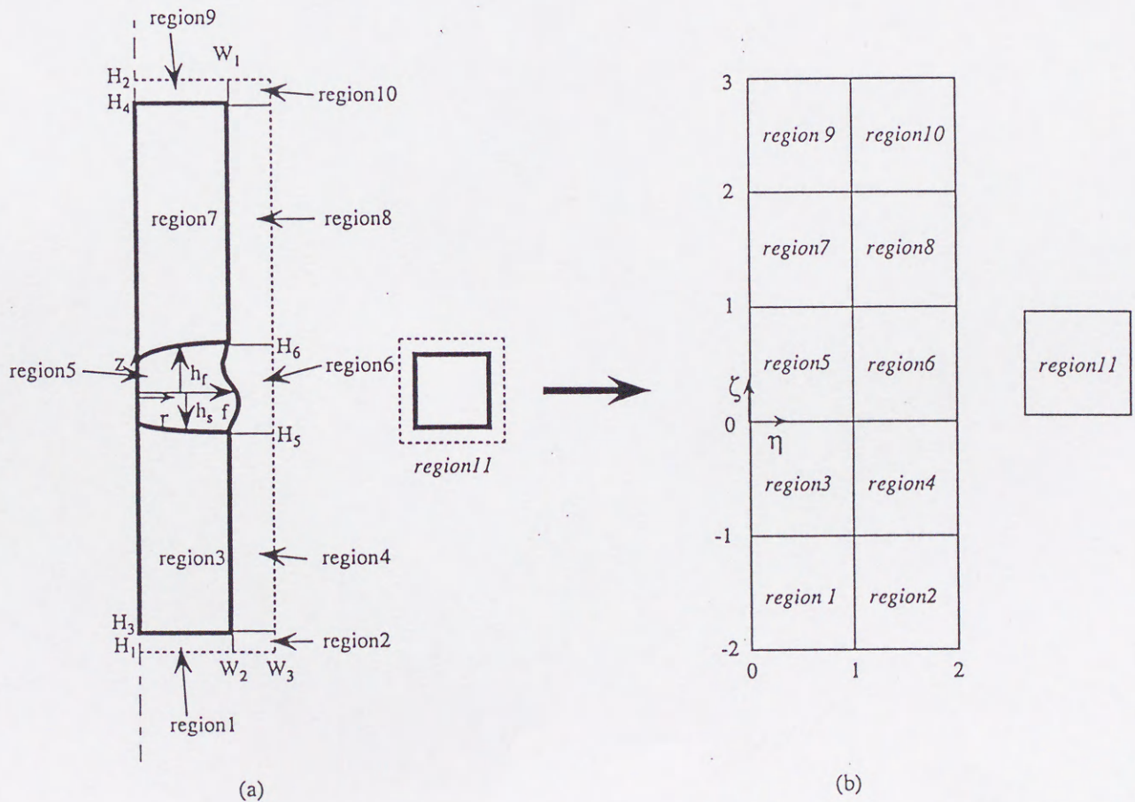
Fig. 3a-1 Schematic diagram of coordinate transformation
