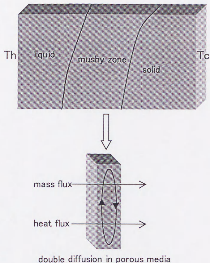
Fig.4-1 Schematic model of solution crystal growth system and the phenomena in mushy zone
