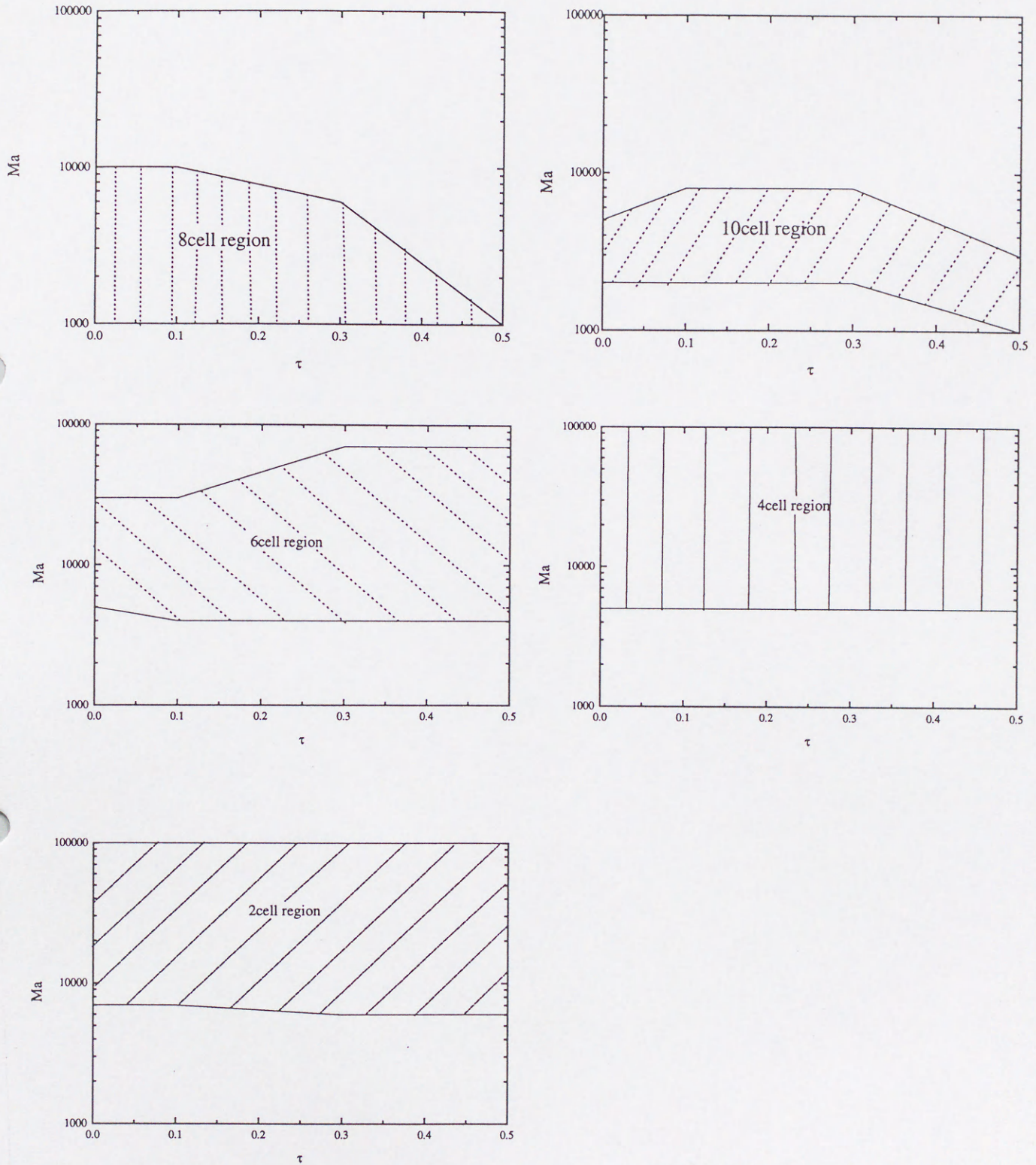
Fig.2-11 The range of stable solution for each convection cell pattern with and without inner heating
