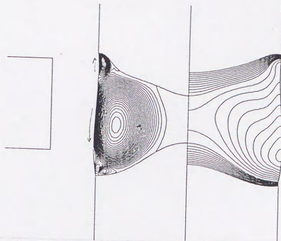
Fig.3-12 Effect of MHD and Marangoni convection when N_Q=3.89 \times 10^5 , N_A=3.32 \times 10^2 , N_F=8.44 \times 10^8 and Ma=5.0 \times 10^6
