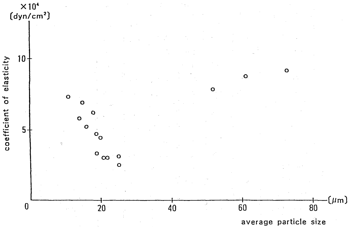
Fig.1 Effect of average particle size after fermentation on the coefficient of elasticity of yogurt
