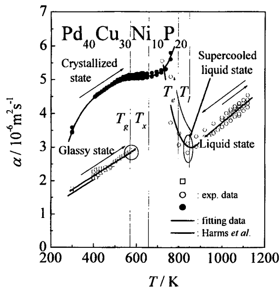
Fig. 1 Thermal diffusivity of Pd 40 Cu 30 Ni 10 P 20 glassy alloy.
